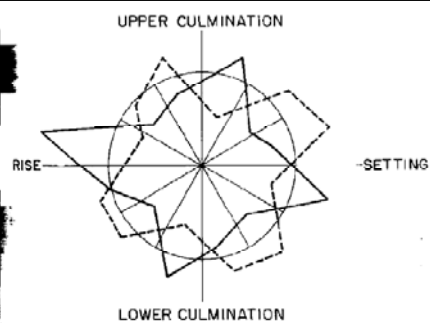
Figure 2. Mars and Strong-willed and Weak-willed Champions Note: the mean number of champions born with Mars in each part of its daily orbit. Continuous lines: strong-willed champions are born more often just after Mars has risen or set. Broken lines: weak-willed champions are born less often with Mars in these positions
